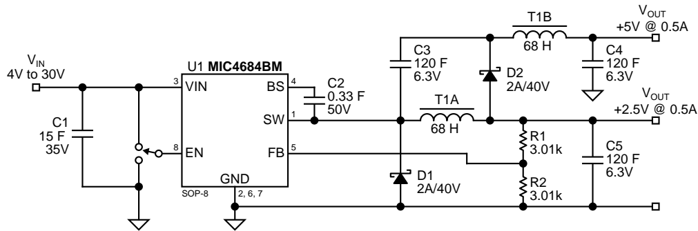
Figure 1. 2.5V and 5.0V Stacked Winding Output
