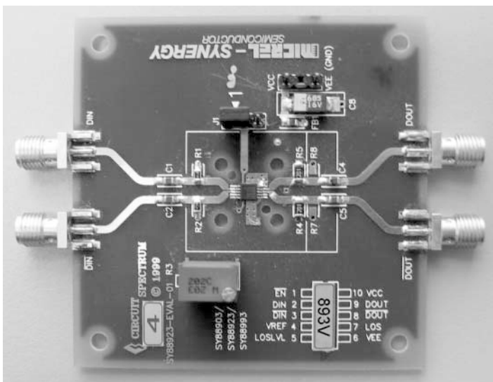
Figure 1. SY88893V Evaluation Board
