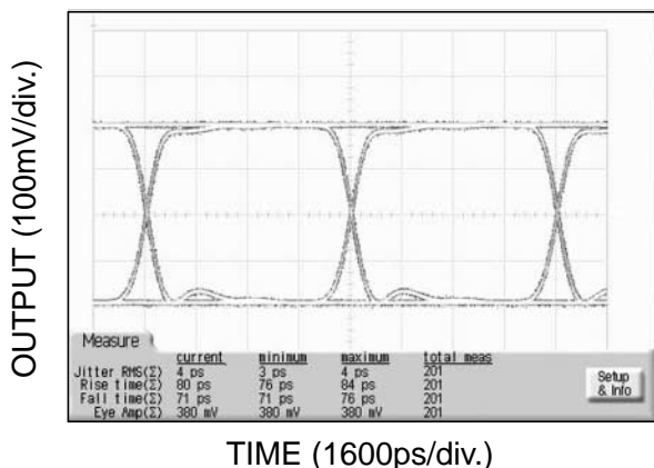
Figure 3. Typical SY88893V Eye Diagram
