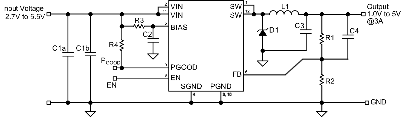
MIC2207 Schematic
